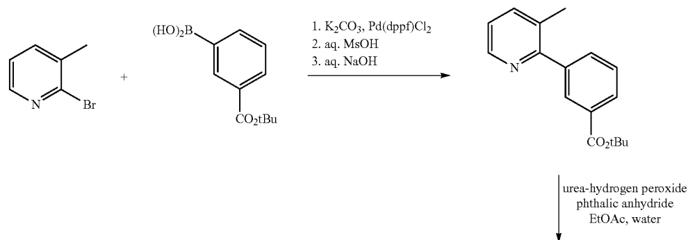
Scheme 3. Synthesis of the amine moiety.
