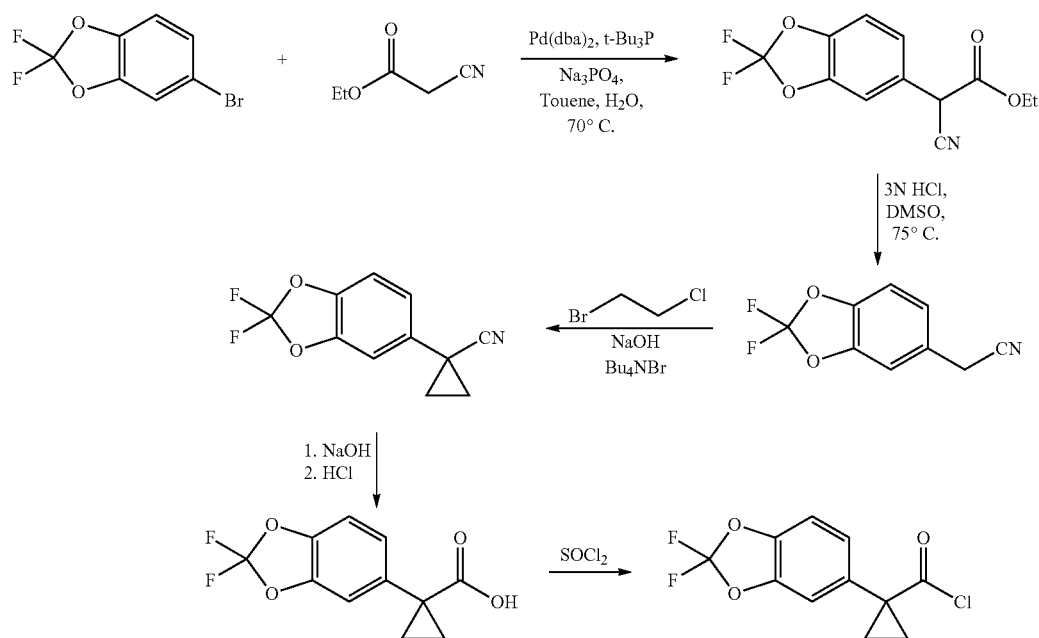
Scheme 2. Alternative synthesis of the acid chloride moiety.
