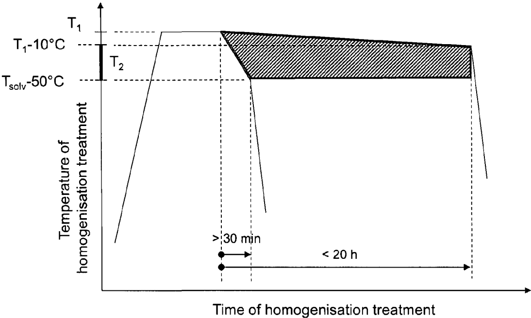
Sketch of a temperature-time chart for homogenisation where the shaded area indicates the temperature-time window encompassed by the invention as defined in the Claims.
