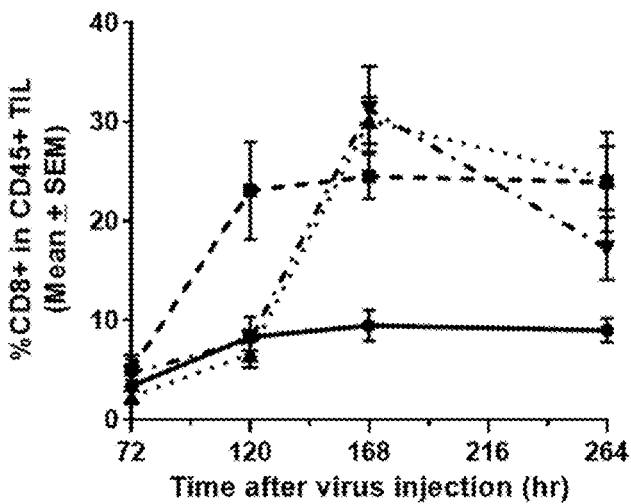
CD8+ T cell kinetics
