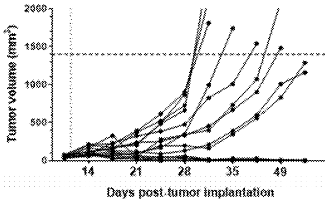
1e7 Cop.mIL-2v.A34-K151E (IT dosing on D10)
