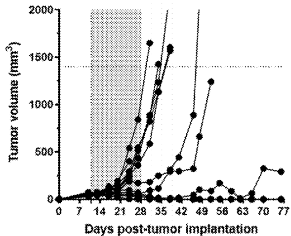
G6: WR.mIL2v.A34-K151E (anti-PD1 mAb Tx)
