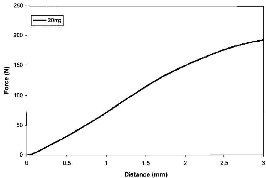
Example 20 Indentation Test of Example 13.3 tablet
