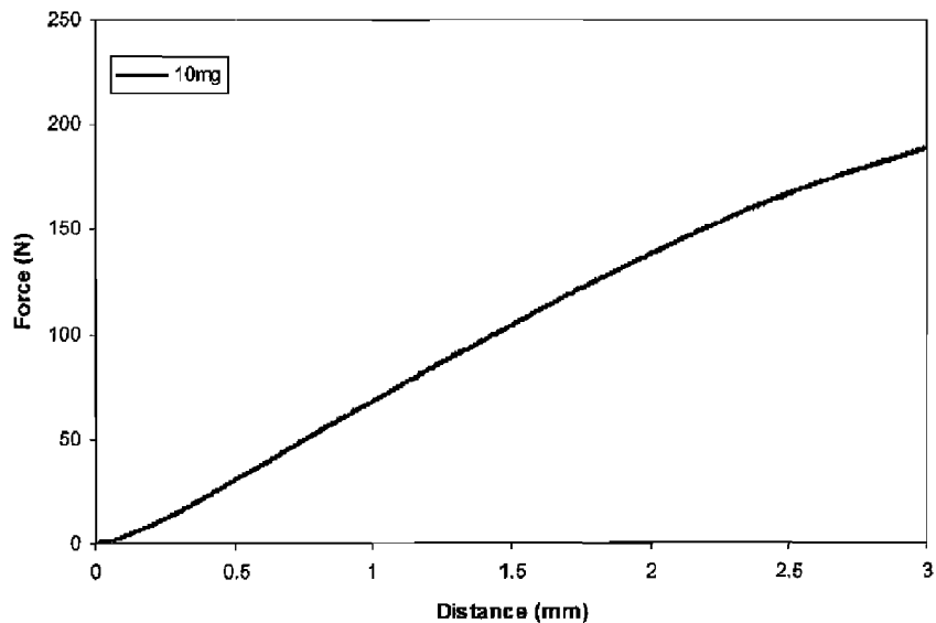
Example 20 Indentation Test of Example 13.1 tablet
