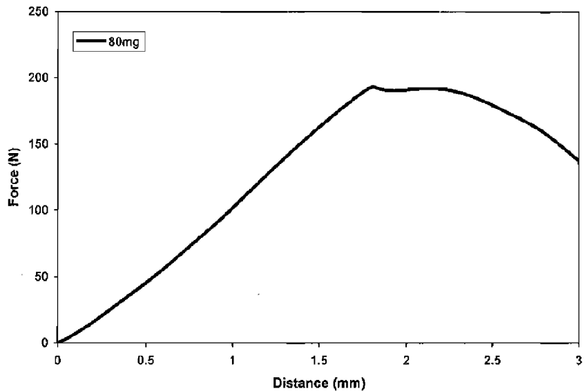
Example 20 Indentation Test of Example 18.2 tablet
