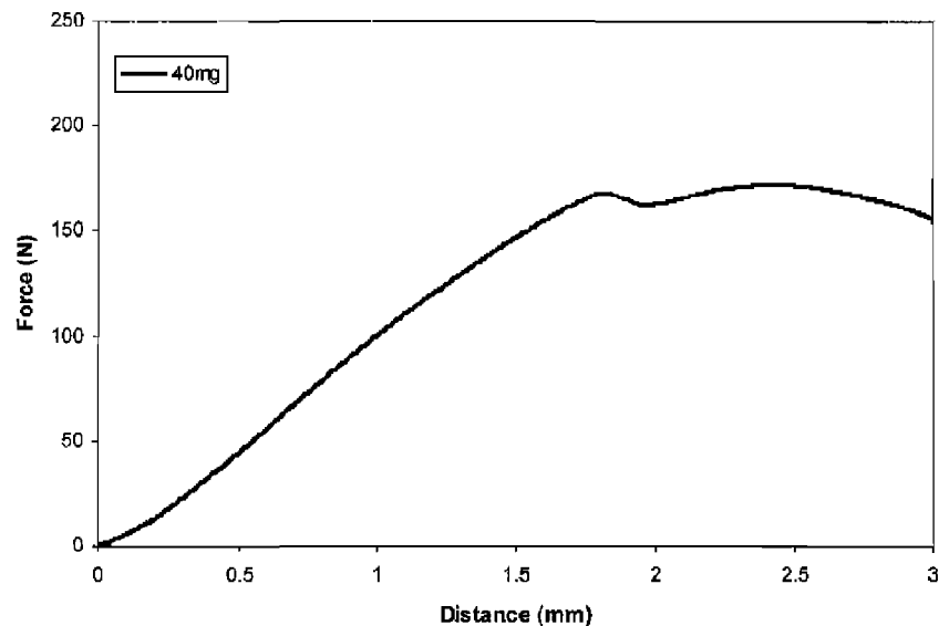
Example 20 Indentation Test of Example 13.5 tablet
