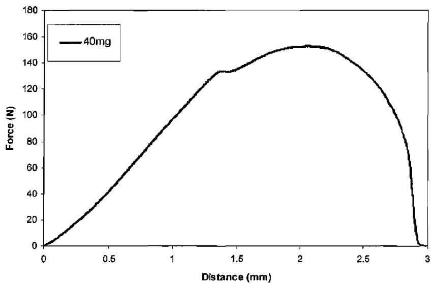
Example 20 Indentation Test of Example 14.5 tablet
