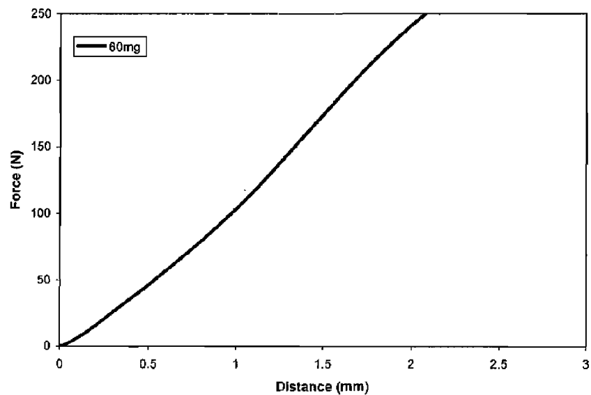
Example 20 Indentation Test of Example 17.1 tablet
