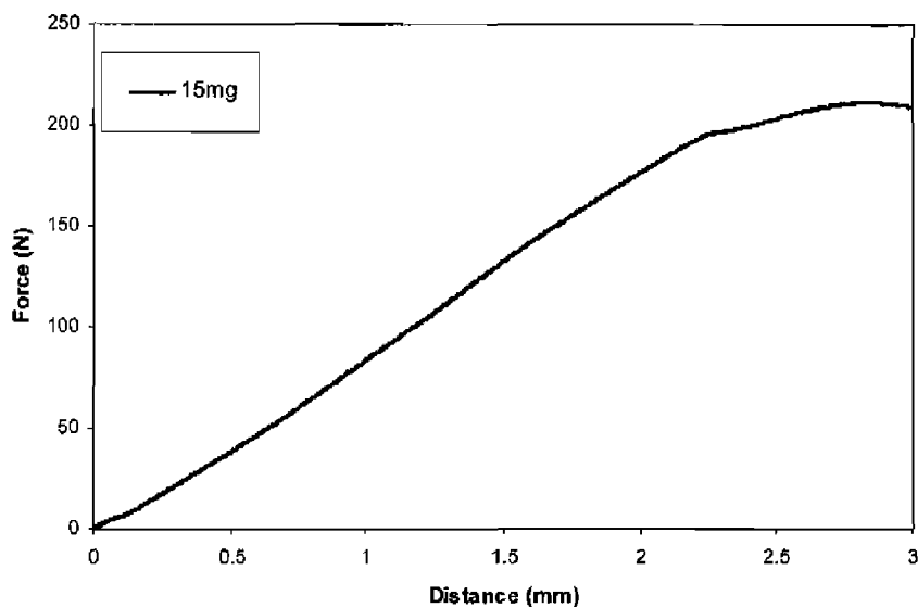
Example 20 Indentation Test of Example 14.2 tablet
