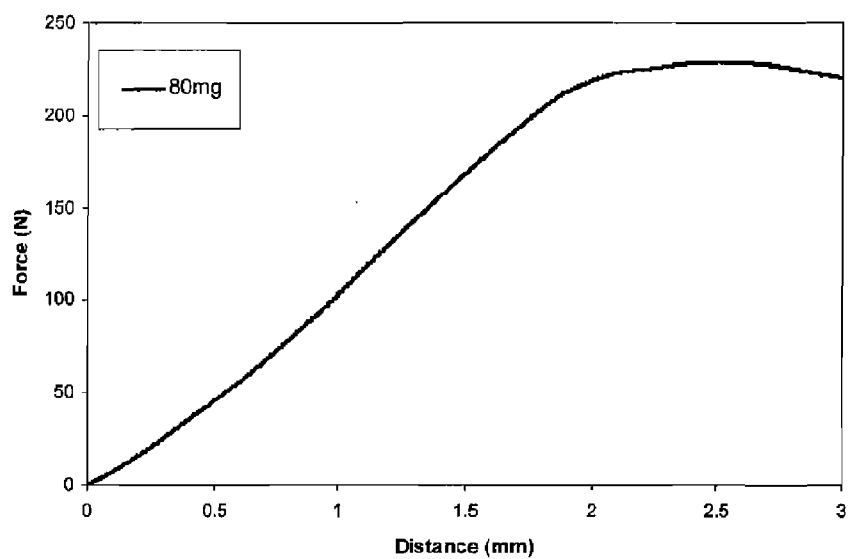
Example 20 Indentation Test of Example 16.2 tablet
