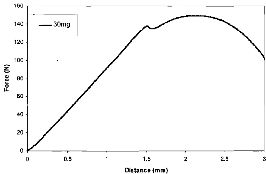
Example 20 Indentation Test of Example 14.4 tablet
