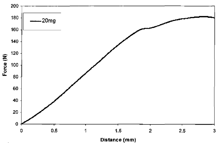
Example 20 Indentation Test of Example 14.3 tablet
