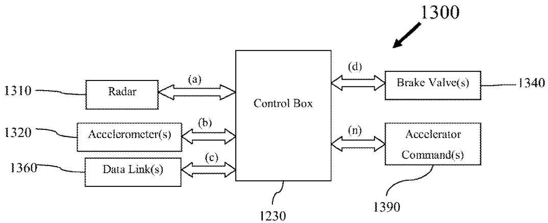
Figure 12: Simplified system block diagram
