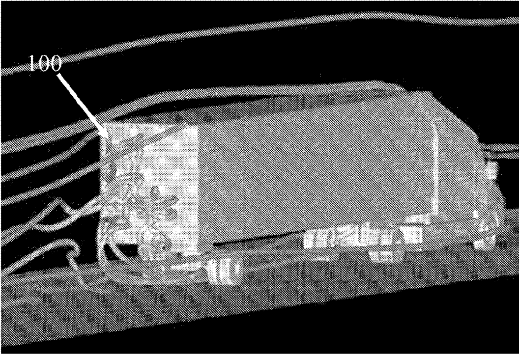
Figure 1: Airflow Around a Heavy Truck.
