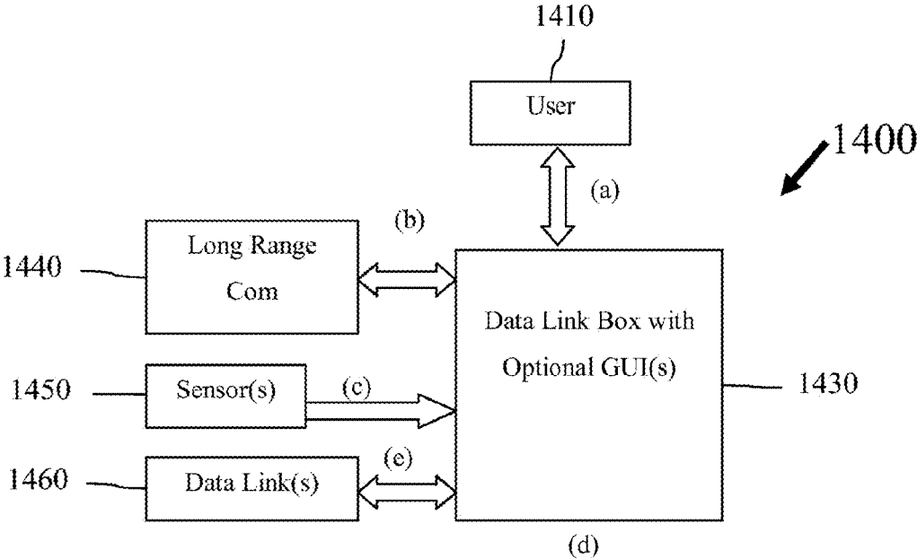
Figure 14: Simplified System for Lead Vehicle
