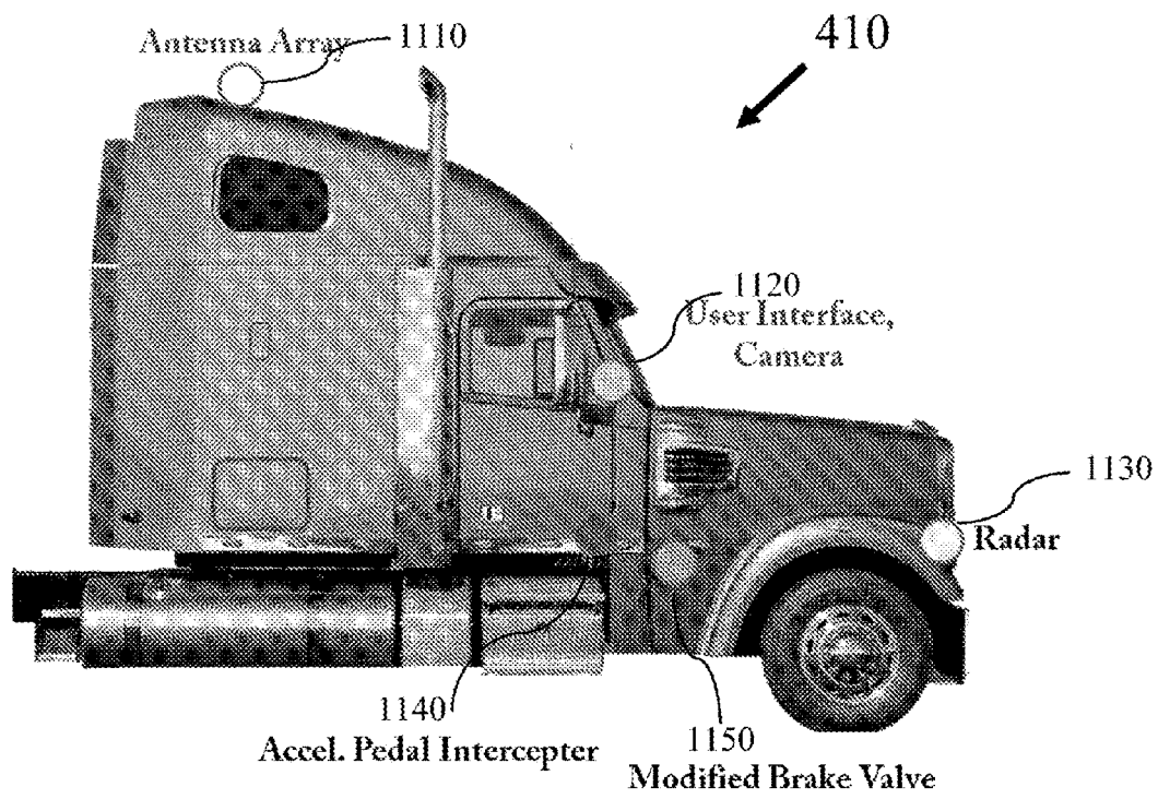
Figure 11: Possible list of system components.
