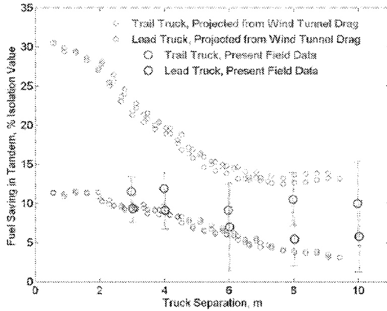
Figure 5: Fuel savings versus vehicle gap (Heavy Trucks)
