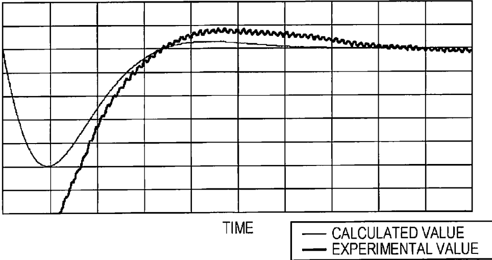
FIG. 11 EXPERIMENTAL VALUE AND CALCULATED VALUE OF RESIDUAL VIBRATION (DRIED)
