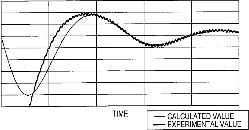
EXPERIMENTAL VALUE AND CALCULATED VALUE OF RESIDUAL VIBRATION (NORMAL STATE)
