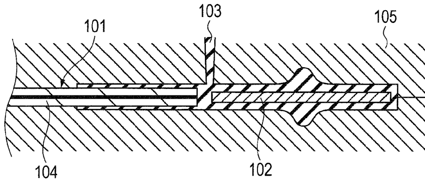
FIG. 11 PRIOR ART
