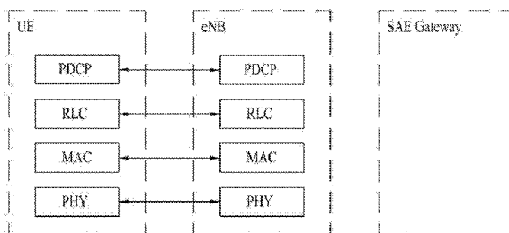
(b) User-plane protocol stack
