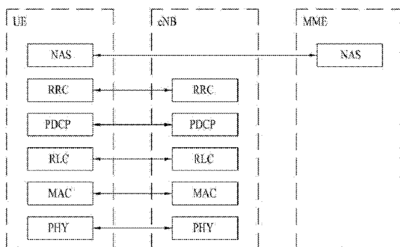
(a) Control-plane protocol stack
