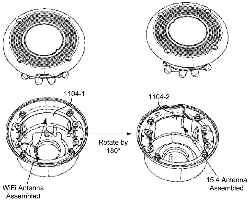
Antenna Placement inside the Camera Module
