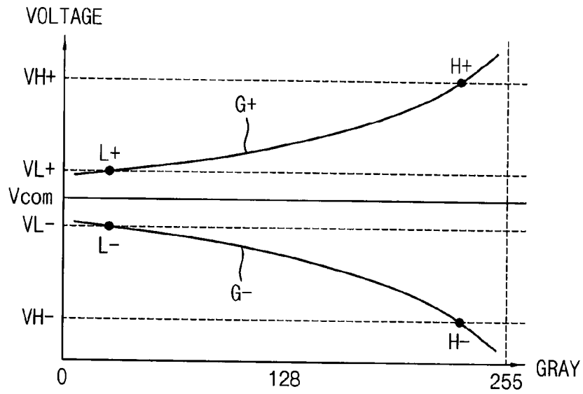
FIG. 4 (RELATED ART)
