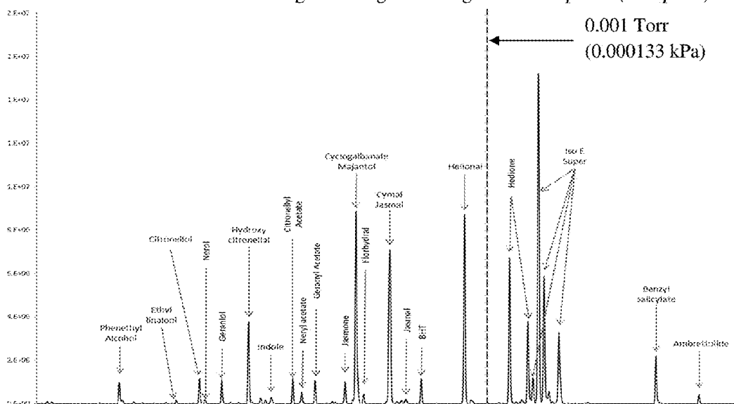
Figure 22(a)(i) – Headspace Chromatography – After 10 mins Evaporation No Modulator & Traditional Muguesia Magnifica Fragrance Example 5a (Comp. L2)
