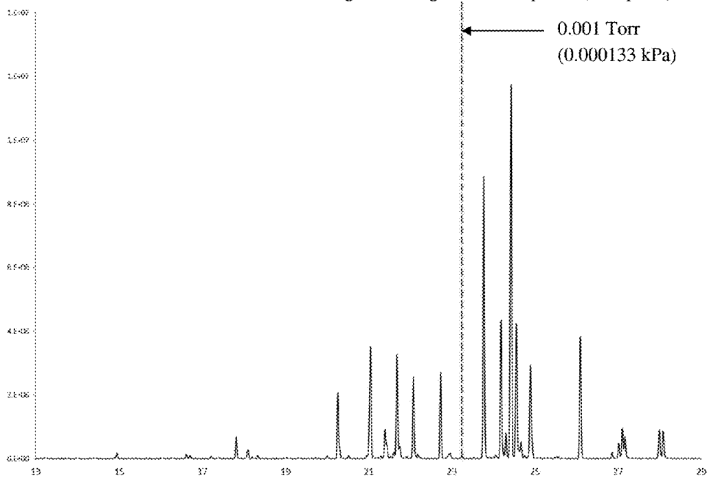
Figure 24(a)(ii) – Headspace Chromatography – After 60 mins Evaporation No Modulator & Traditional Floral Magnifica Fragrance Example 4a (Comp. L4)
