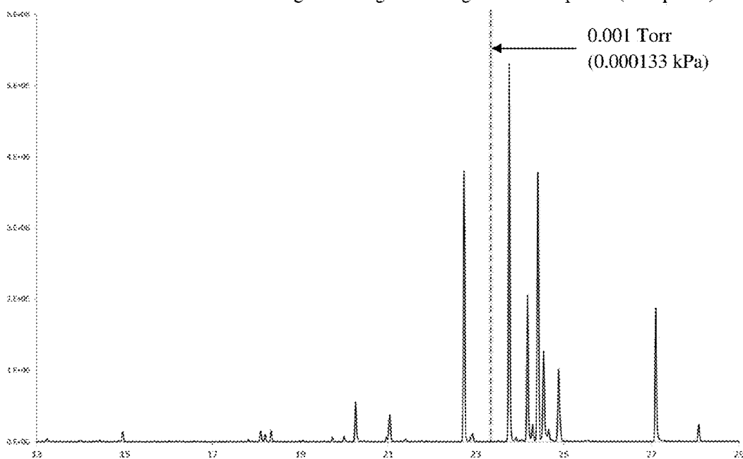
Figure 22(a)(ii) – Headspace Chromatography – After 60 mins Evaporation No Modulator & Traditional Muguesia Magnifica Fragrance Example 5a (Comp. L2)
