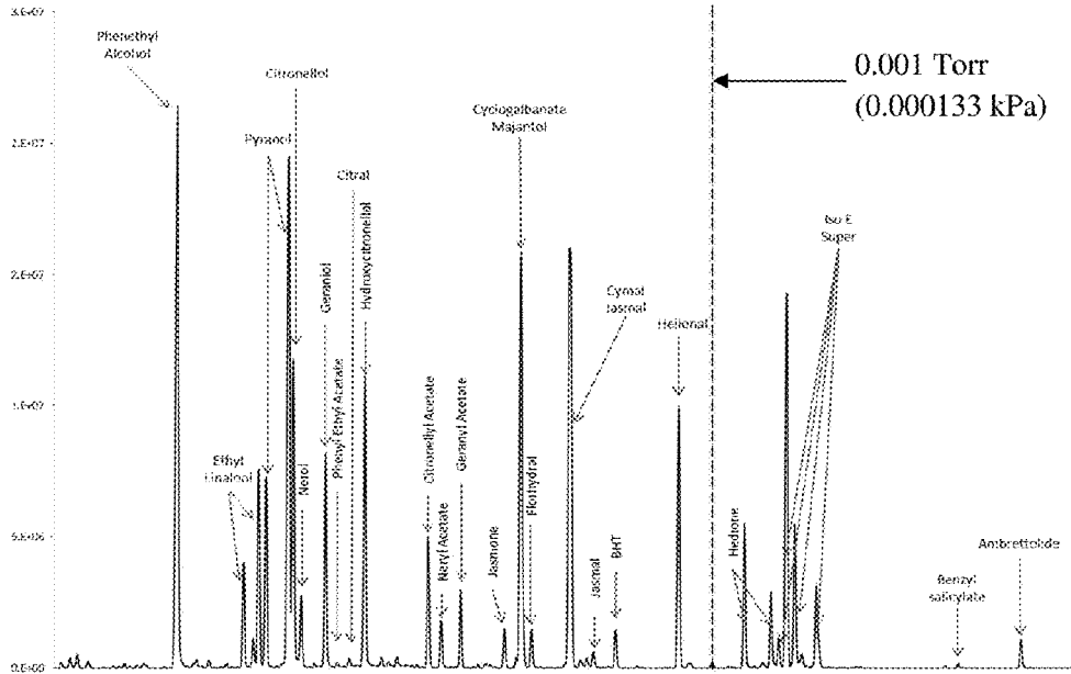
Figure 25(b)(i) – Headspace Chromatography – After 10 mins Evaporation Undecyl Glucoside (i.e., Simulsol® SL 11W/ Modulator) & Diamond Muguesia Magnifica Fragrance Example 5b (Comp. G4)
