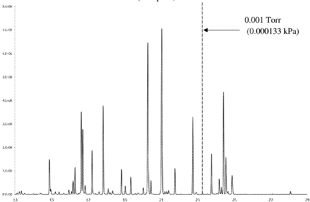
Figure 22(b)(ii) – Headspace Chromatography – After 60 mins Evaporation PPG-11 Stearyl Ether (Modulator) & Diamond Muguesia Magnifica Fragrance Example 5b (Comp. J2)
