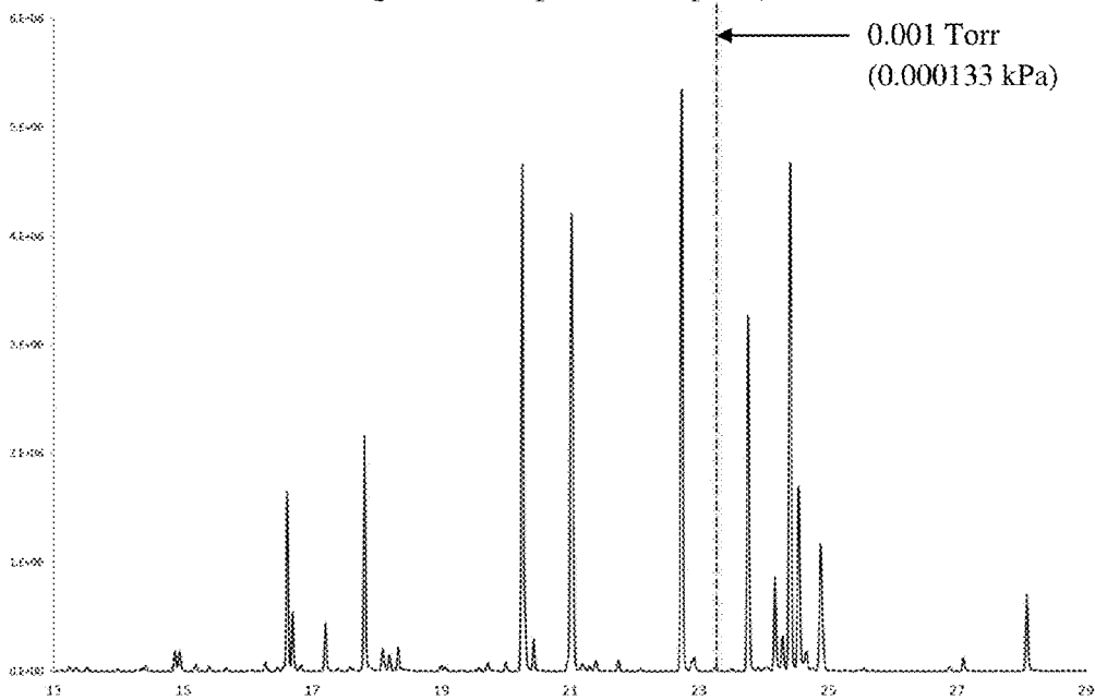
Figure 25(b)(ii) – Headspace Chromatography – After 60 mins Evaporation Undecyl Glucoside (i.e., Simulsol® SL 11W/ Modulator) & Diamond Muguesia Magnifica Fragrance Example 5b (Comp. G4)
