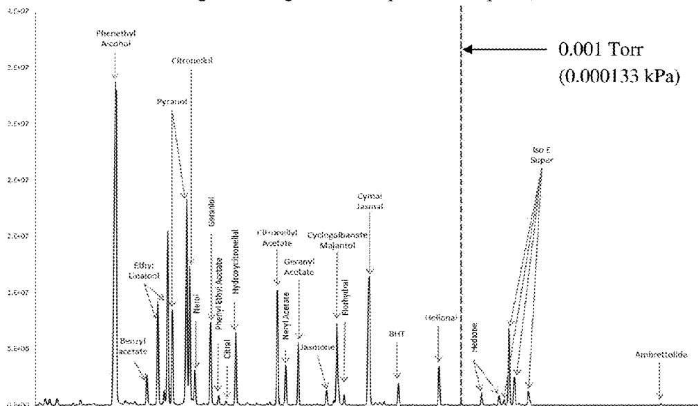
Figure 23(b)(i) – Headspace Chromatography – After 10 mins Evaporation PPG-20 Methyl Glucose Ether (i.e., GLUCAM™ P-20/ Modulator) & Diamond Muguesia Magnifica Fragrance Example 5b (Comp. A4)
