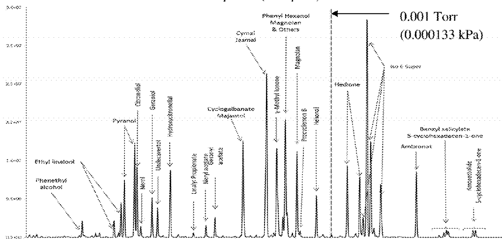
Figure 24(b)(i) – Headspace Chromatography – After 10 mins Evaporation Isocetyl Alcohol (i.e., Ceraphyl ® ICA/ Modulator) & Diamond Floral Magnifica Fragrance Example 4b (Comp. J4)
