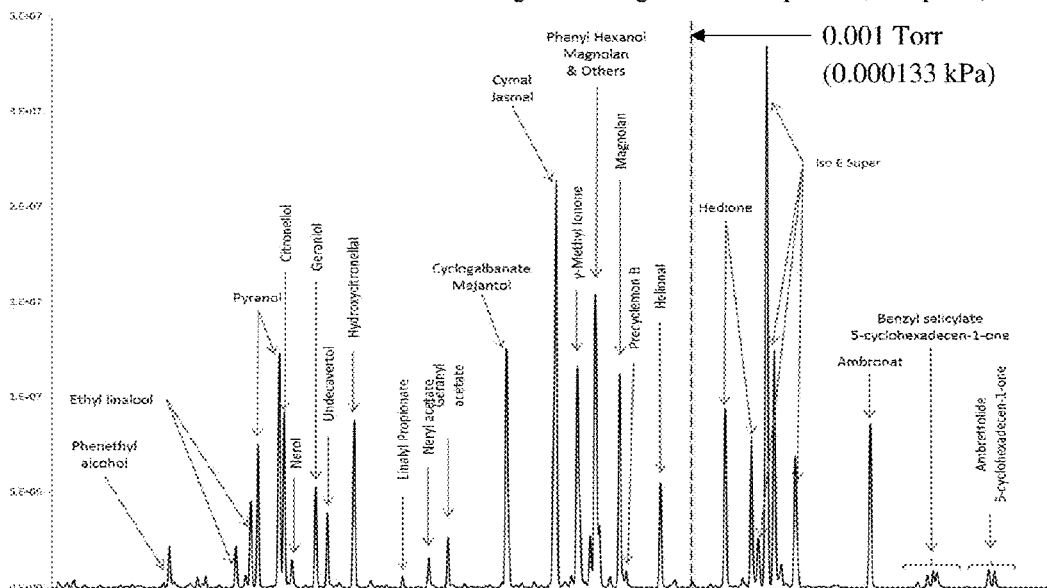
Figure 24(a)(i) – Headspace Chromatography – After 10 mins Evaporation No Modulator & Traditional Floral Magnifica Fragrance Example 4a (Comp. L4)
