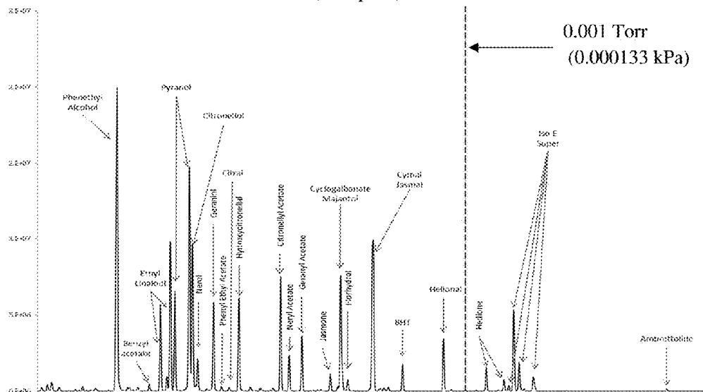
Figure 22(b)(i) – Headspace Chromatography – After 10 mins Evaporation PPG-11 Stearyl Ether (Modulator) & Diamond Muguesia Magnifica Fragrance Example 5b (Comp. J2)
