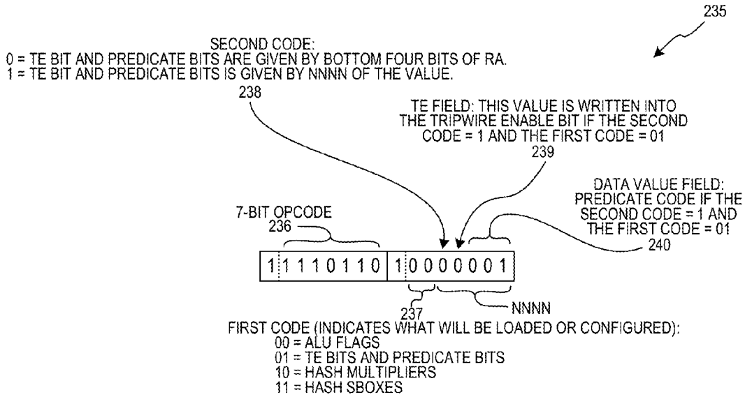
LOAD REGISTER FILE READ STAGE CONTROL REGISTER INSTRUCTION
