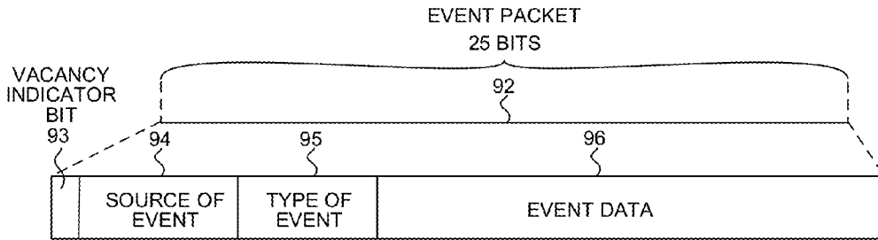
EVENT PACKET BIT SEQUENCE
