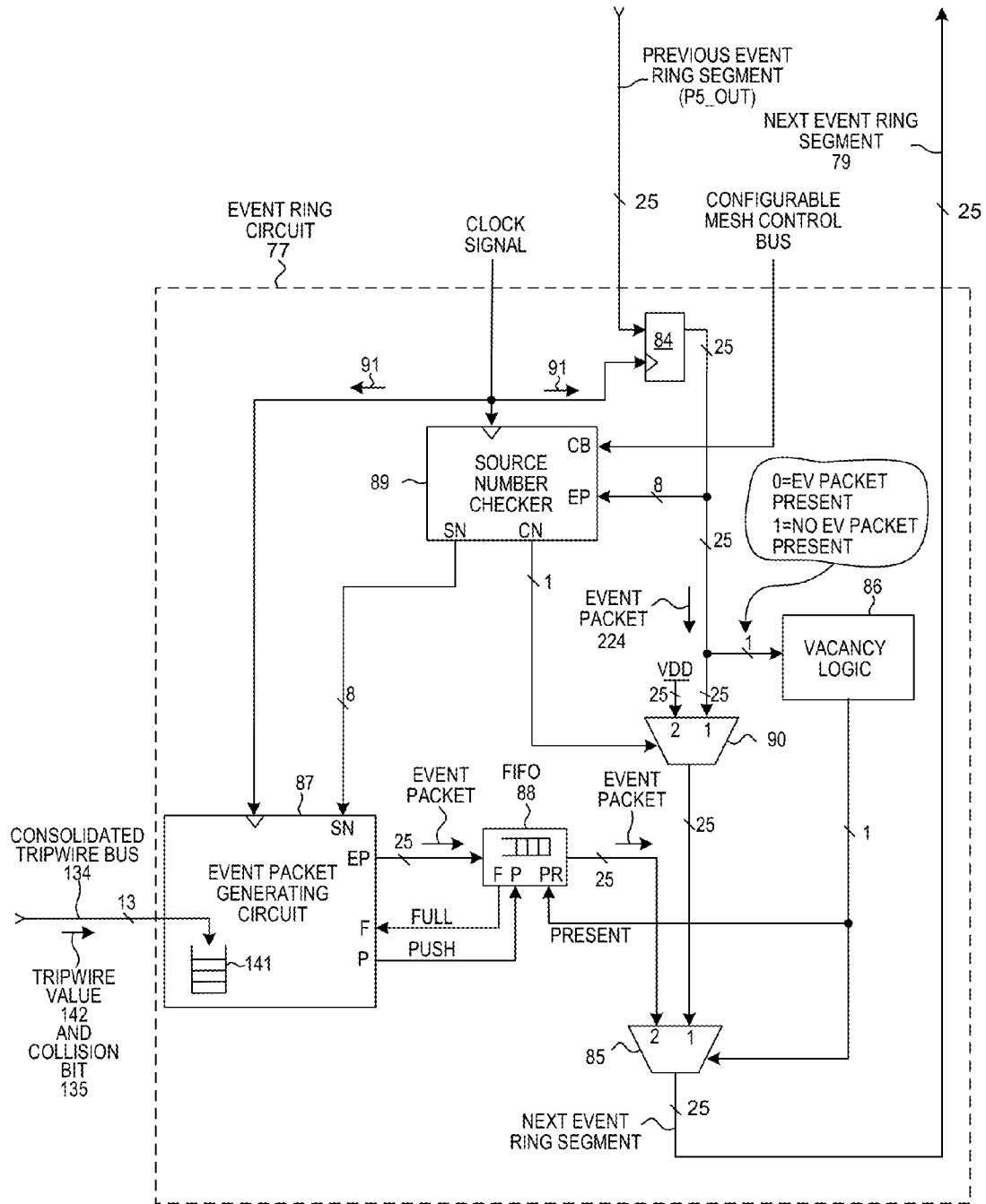
EVENT RING CIRCUIT FIG. 5
