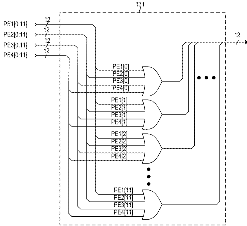
12x4:1 OR STRUCTURE
