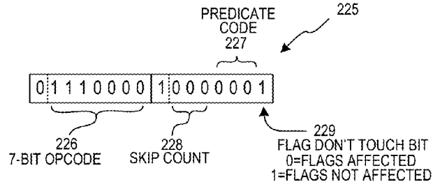
SKIP INSTRUCTION FIG. 25
