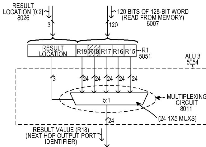
DIRECT 24-BIT LOOK-UP STAGE FIG. 49
