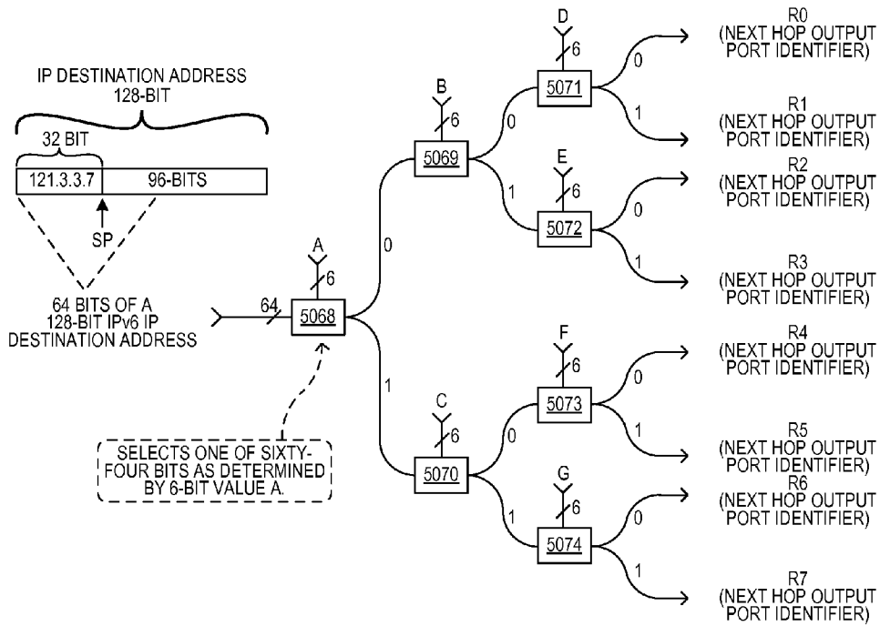
CONCEPTUAL DIAGRAM OF TRIE MULTI-BIT LOOKUP OPERATION
