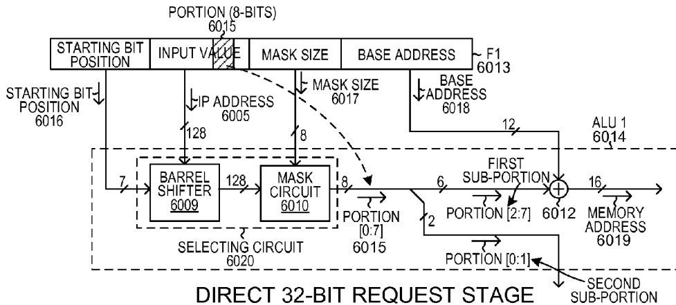
DIRECT 32-BIT MEMORY PACKING SCHEME FIG. 40
