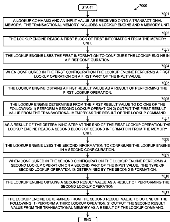
RECURSIVE USE OF MULTIPLE HARDWARE LOOKUP STRUCTURES
