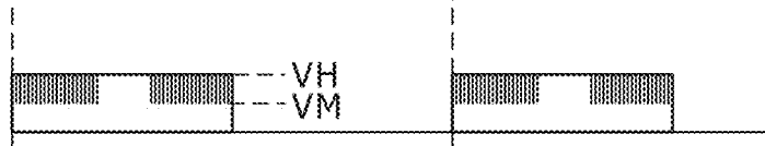
FIG. 39E DUTY40% MOVING IMAGE IMPROVEMENT SYSTEM
