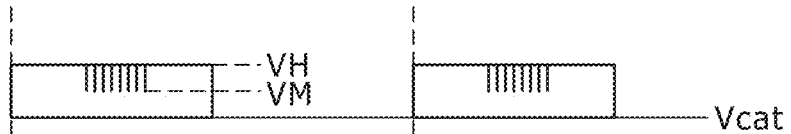
FIG. 39C DUTY45% FLICKER SUPPRESSION SYSTEM
