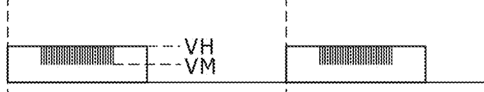
FIG. 39F DUTY30% FLICKER SUPPRESSION SYSTEM
