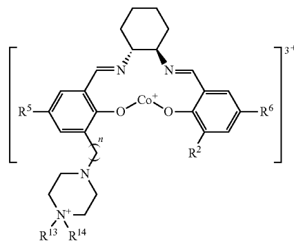
[Chemical Formula 20]
