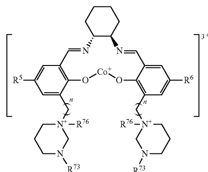
[Chemical Formula 15]
