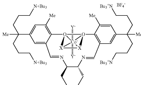
X = 2,4-dinitrophenolate Y = X or [X---H---X]
