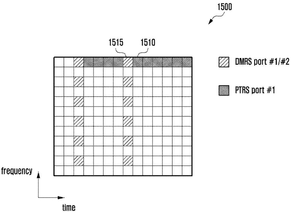
Embodiment in which PTRS is punctured if collision occurs between DMRS and PTRS
