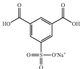
Sodium salt of 5-(sulfo)isophthalic acid (SSIPA)
