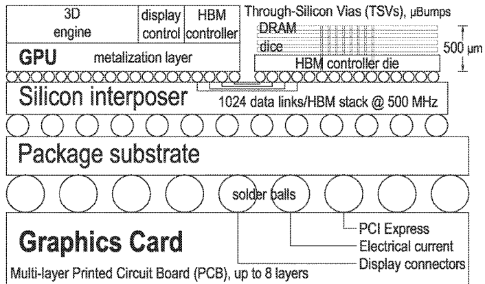
Cross Section of GPU packaged with HBM
