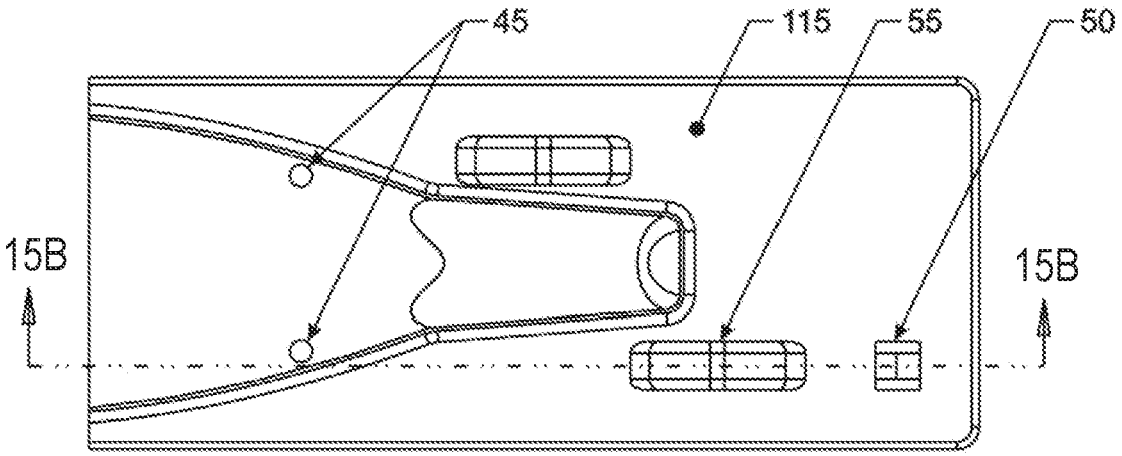
TOP VIEW FIG. 15A
