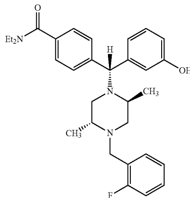
4-((alpha-R)-alpha-((2S,5R)-2,5-dimethyl-4-(2-fluorobenzyl)-1-piperazinyl)-3-hydroxybenzyl)-N,N-diethylbenzamide
