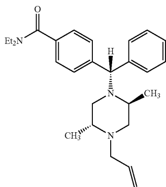
4-((alpha-S)-alpha-((2S,5R)-4-Allyl-2,5-dimethyl-1-piperazinyl)benzyl)-N,N-diethylbenzamide
