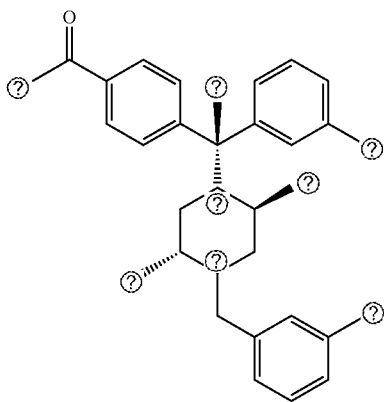
N,N-Diethyl-3-[(R)-[(2S,5R)-4-(3-methoxybenzyl)-2,5-dimethylpiperazin-1-yl] (3-methoxyphenyl)-methyl]benzamide
