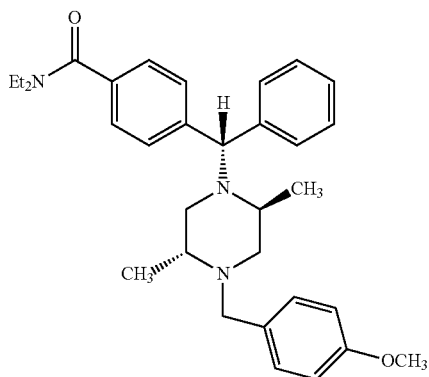
4-((alpha-S)-alpha-((2S,5R)-2,5-Dimethyl-4-(4-methoxybenzyl)-1-piperazinyl)benzyl)-N,N-diethylbenzamide
