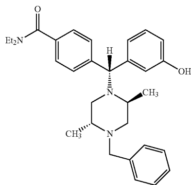
4-((alpha-R)-alpha-((2S,5R)-2,5-Dimethyl-4-(4-fluorobenzyl)-1-piperazinyl)-3-hydroxybenzyl)-N,N-diethylbenzamide
