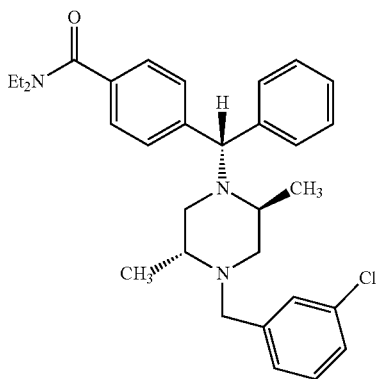
4-((alpha-S)-alpha-((2S,5R)-4-(3-Chlorobenzyl)-2,5-dimethyl-1-piperazinyl)benzyl)-N,N-diethylbenzamide
