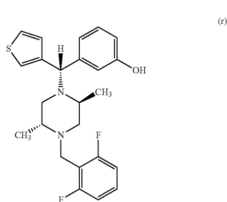
N,N-Diethyl-3-((R)-((2S,5R)-2,5-dimethyl-4-(3-hydroxybenzyl)piperazin-1-yl)(3-hydroxyphenyl)methyl)benzamide
