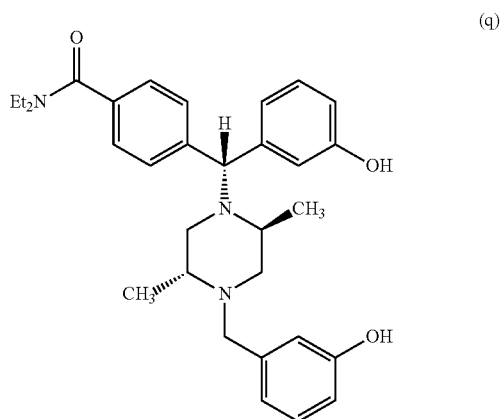
N,N-Diethyl-3-((R)-((2S,5R)-2,5-dimethyl-4-(3-hydroxybenzyl)piperazin-1-yl)(3-hydroxyphenyl)methyl)benzamide
