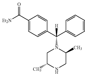
4-((alpha-S)-alpha-((2S,5R)-2,5-dimethyl-1-piperazinyl)benzyl)-N,N-diethylbenzamide
