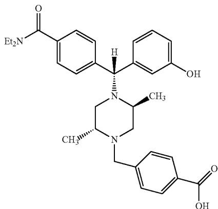
4-((2R,5S)-4-[(R)-(4-Diethylcarbamoylphenyl)(3-hydroxyphenyl)methyl]-2,5-dimethylpiperazin-1-ylmethyl)benzoic acid
