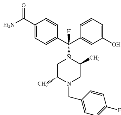
4-((alpha-R)-alpha-((2S,5R)-2,5-Dimethyl-4-(4-fluorobenzyl)-1-piperazinyl)-3-hydroxybenzyl)-N,N-diethylbenzamide
