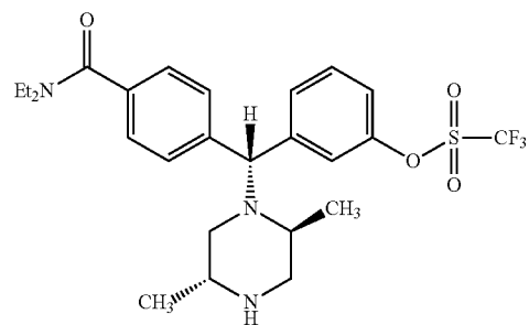
4-((alpha-R)-alpha-((2S,5R)-2,5-Dimethyl-1-piperazinyl)-3-trifluoromethylsulfonyloxybenzyl)-N,N-diethylbenzamide
