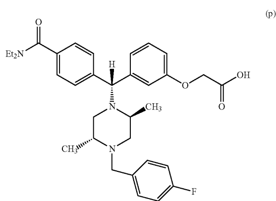
3-((alpha-R)-4-(Diethylaminocarbonyl)-alpha-((2S,5R)-2,5-dimethyl-4-(4-fluorobenzyl)-1-piperazinyl)benzyl)phenoxyacetic acid
