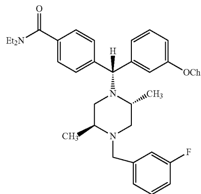
4-((alpha-S)-alpha-((2R,5S)-2,5-Dimethyl-4-(3-fluorobenzyl)-1-piperazinyl)benzyl)-N,N-diethylbenzamide and
