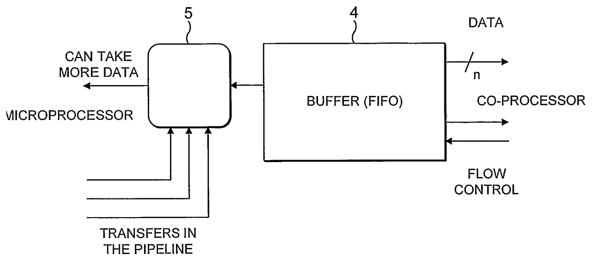
A BUFFERED CO-PROCESSOR INTERFACE
