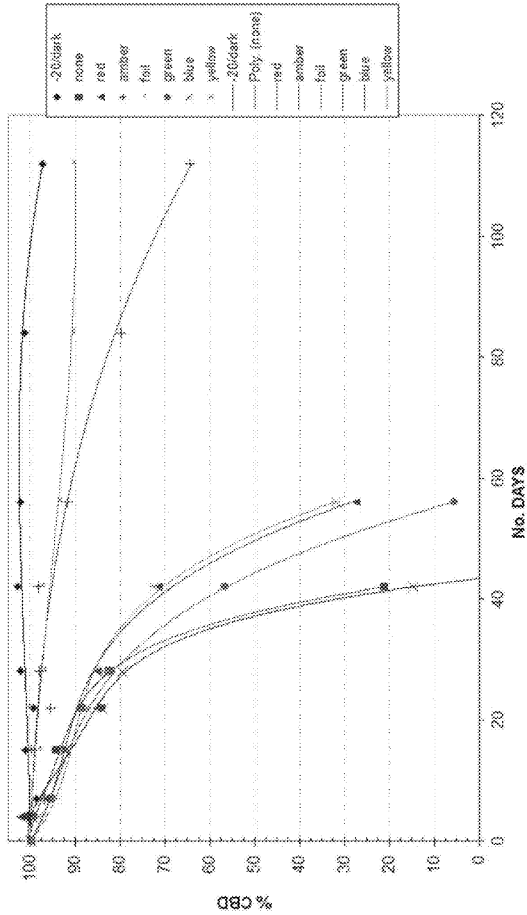
FIGURE 7a. CBD EX CHARCOAL (1 mg/ml soln in MeOH). PHOTOCHEMICAL DEGRADATION. AS012011AX282
