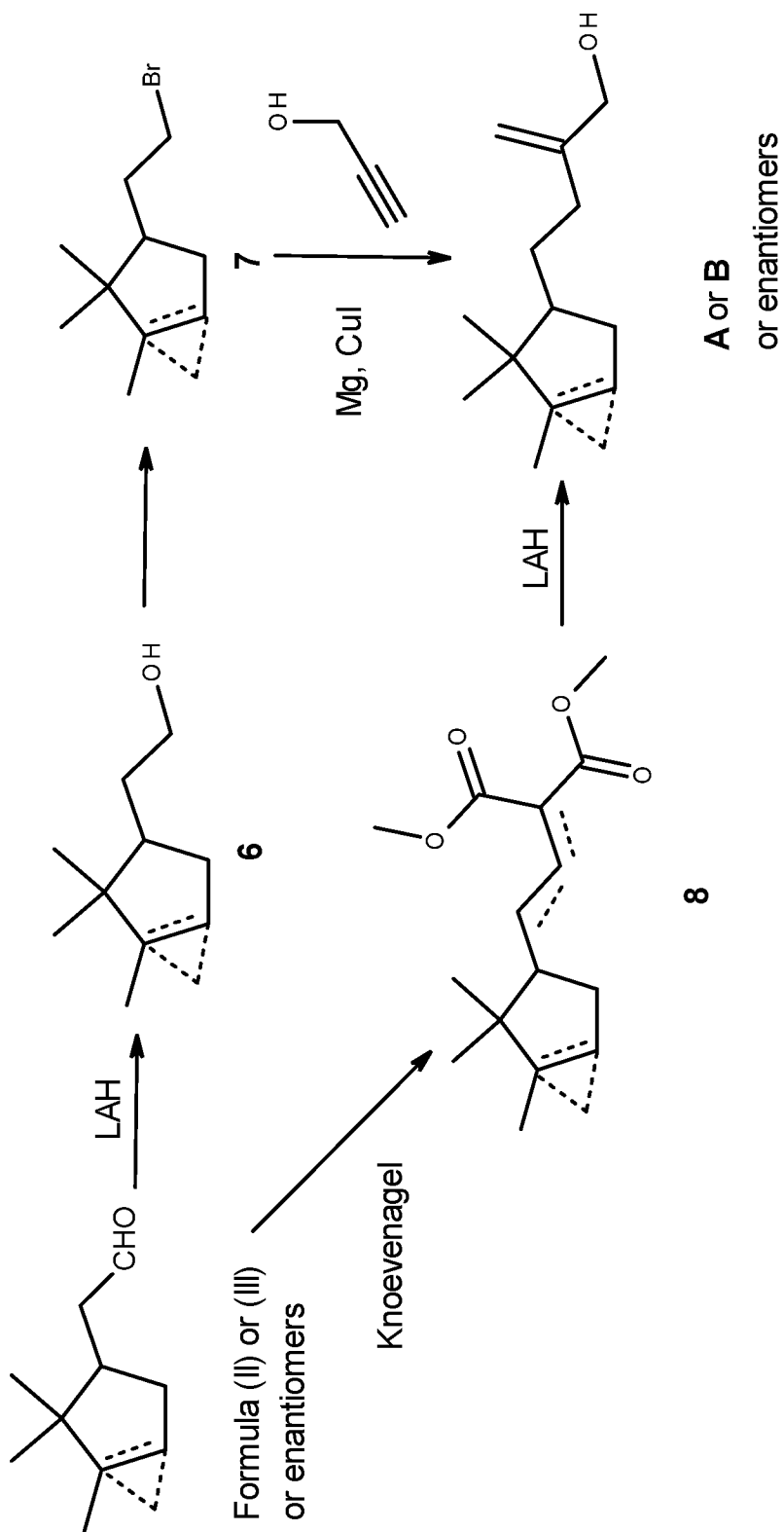
Reaction scheme 3
