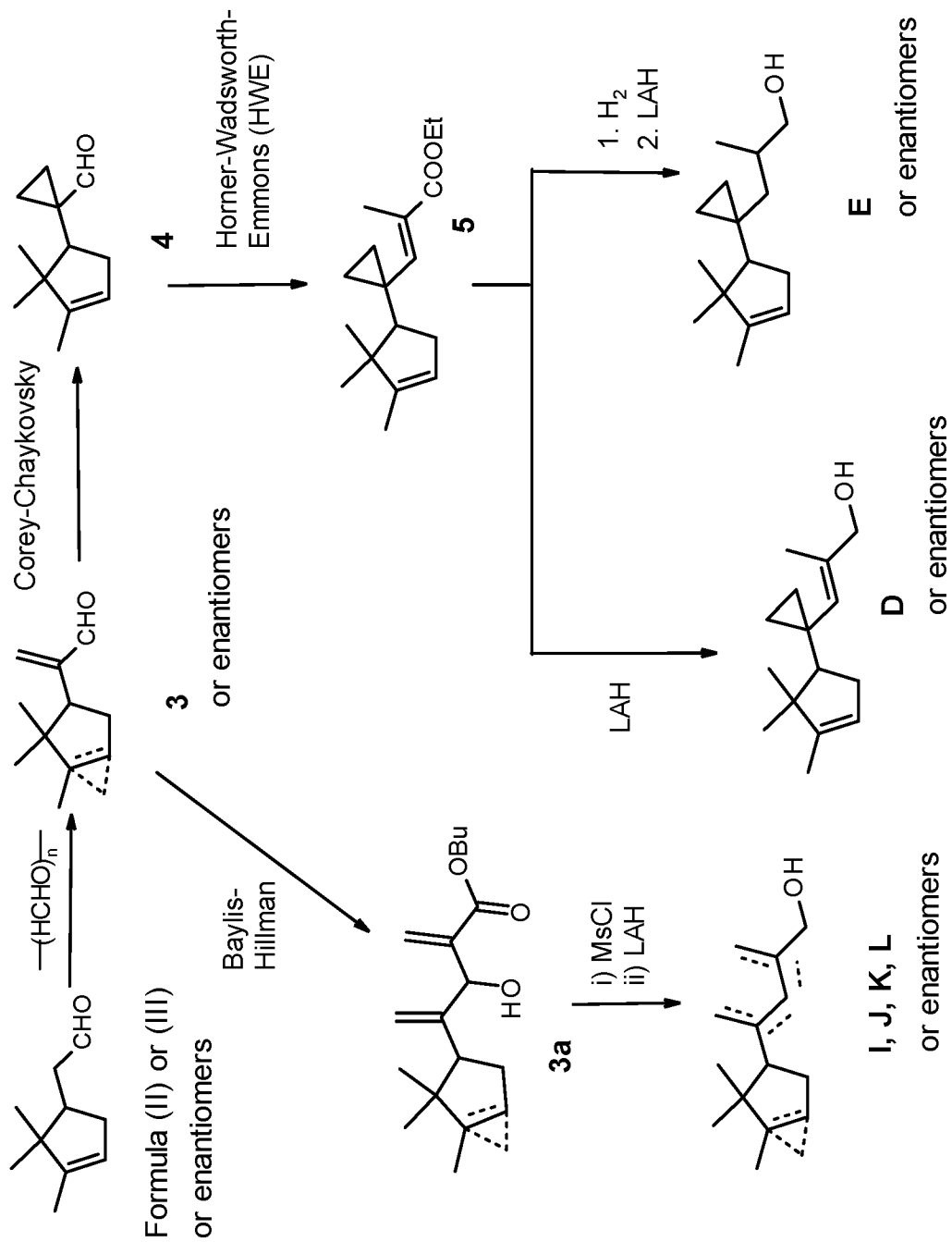
Reaction scheme 2
