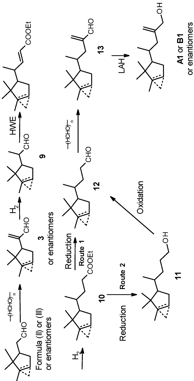
Reaction scheme 4
