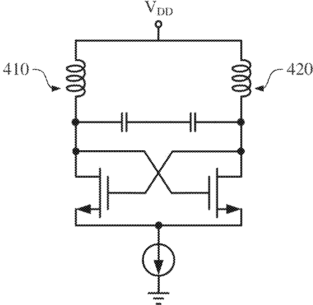
Fig. 4 (prior art)
