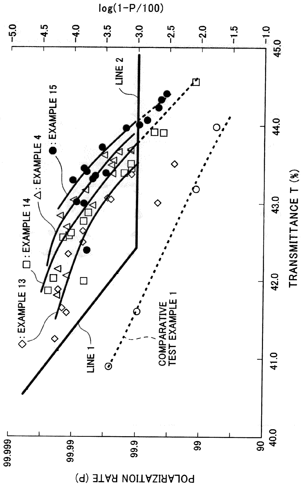
FIG. 16 POLARIZING PROPERTY OF POLARIZING FILM
