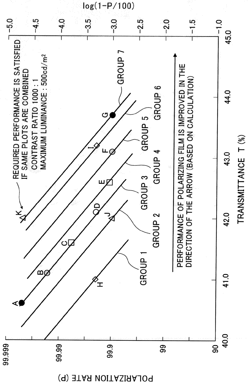
FIG. 5 POLARIZING PROPERTY OF POLARIZING FILM
