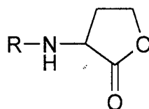
N-acyl-L-homoserine lactone
