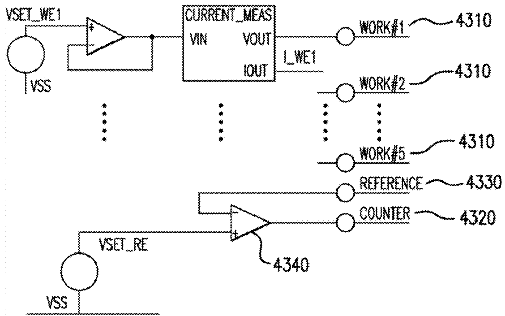
POTENTIOSTAT CONFIGURATION
