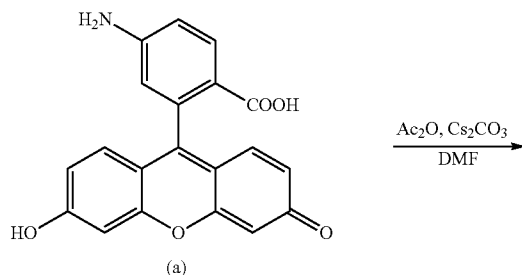
Compound 4
