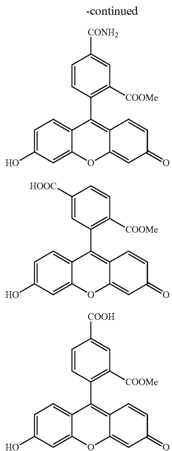
Compound 4
