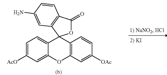
Compound 5
