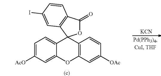
Compound 6
