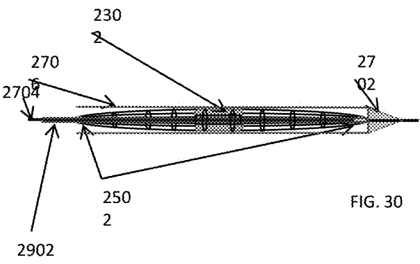
Delivery method for a magnet free floating in a lantern-shape stent
