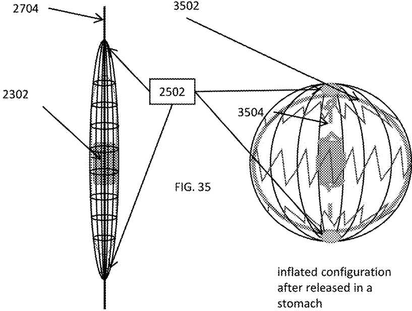
Magnet fixed at the center of a pre-inflated, pre-sealed balloon inside the lantern-shaped structure
