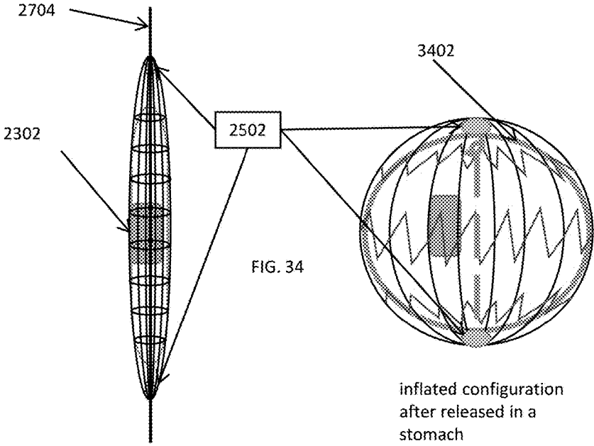
Magnet free-floating in a pre-inflated, pre-sealed balloon inside the lantern-shaped structure
