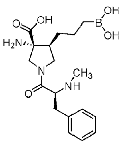
N-methyl phenylalanine AUC = 262
