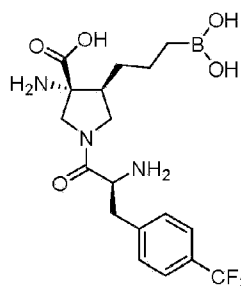
Trifluoromethyl phenylalanine AUC = 5783
