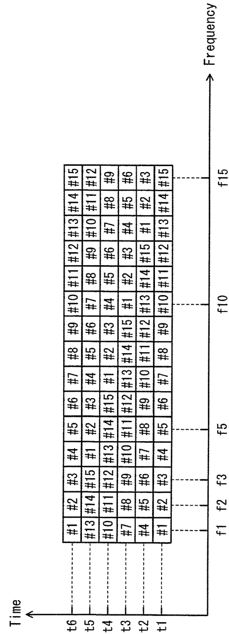
FIG. 76B Modulated signal z2
