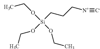
Chemical Formula 2
