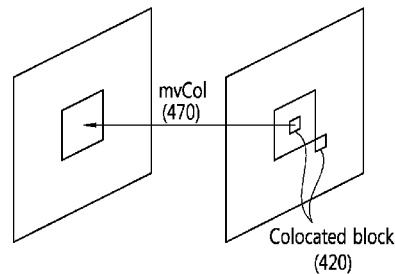
reference picture of Colocated block (440)
