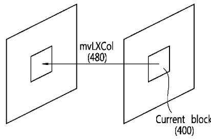
reference picture of Current Picture reference index of temporal merging candidate (460)
