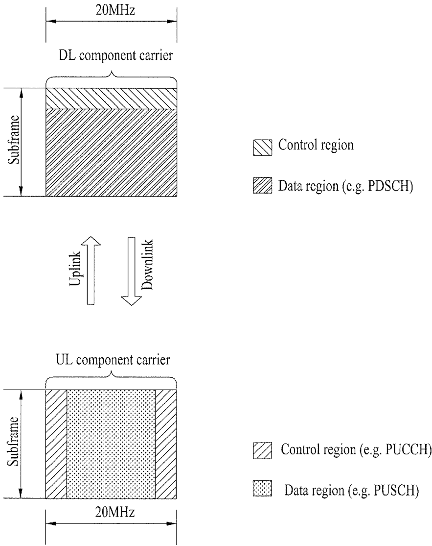
Single component carrier (e.g. LTE system)
