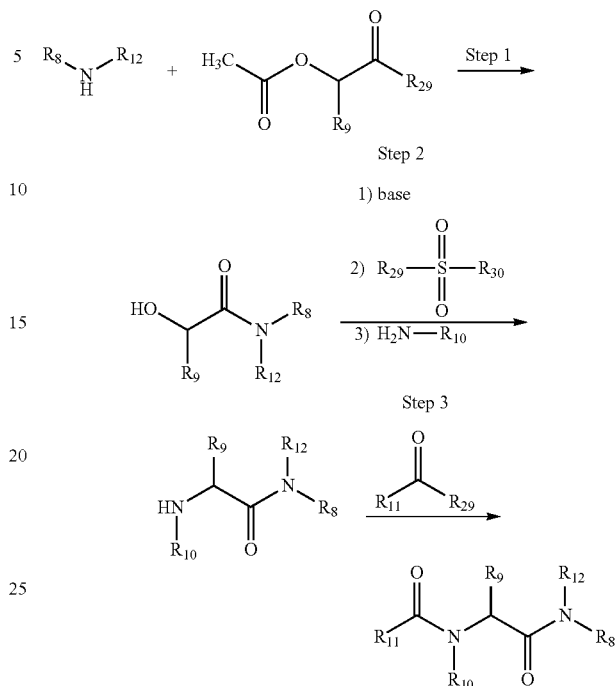
Scheme VII: Formation of compounds represented by Formula III.
