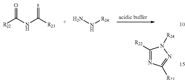
Scheme V: Formation of a triazole.
