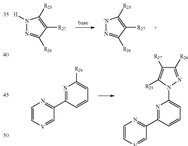
Scheme IV: Formation of a substitute 1-(pyridin-2-yl)pyrazole.
