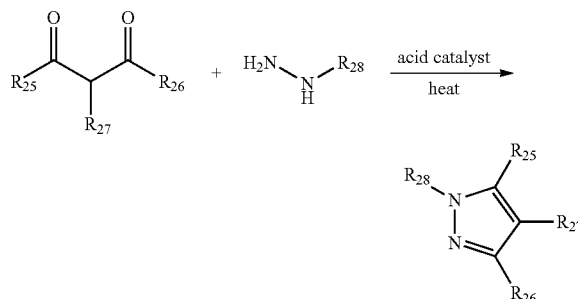
Scheme I: Formation of pyrazole ring.
