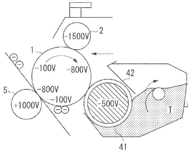
IMAGE FORMING OPERATION
