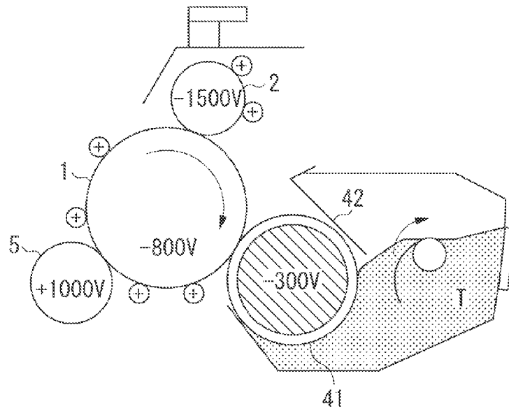
DEVELOPER SUPPLY OPERATION PRIOR TO IMAGE FORMING OPERATION
