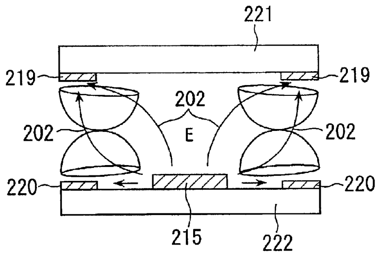
PRIOR ART
