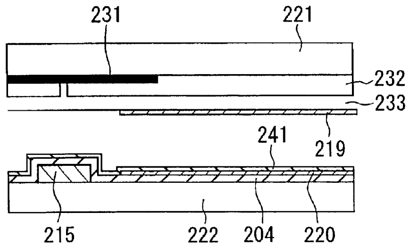
PRIOR ART
