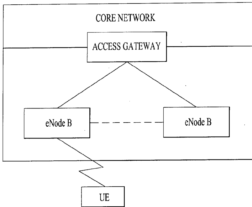
E-UMTS
