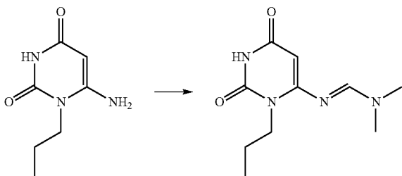
N-(2,6-Dioxo-3-propyl-1,2,3,6-tetrahydro-pyrimidin-4-yl)-N,N-dimethyl-formamide
