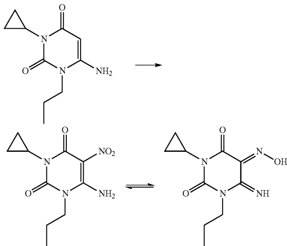
6-Amino-3-cyclopropyl-5-nitroso-1-propyl-1H-pyrimidine-2,4-dione
