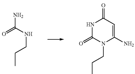
6-Amino-1-propyl-1H-pyrimidine-2,4-dione
