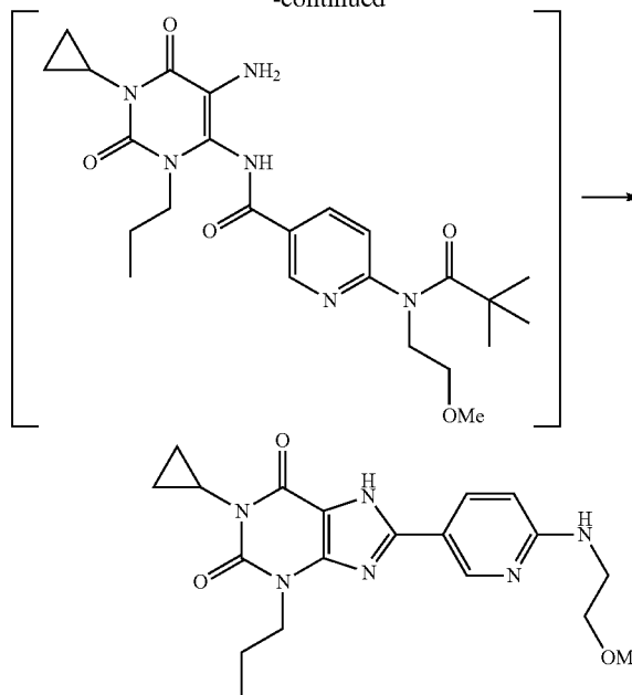
1-Cyclopropyl-8-[6-(2-methoxy-ethylamino)-pyridin-3-yl]-3-propyl-3,7-dihydro-purine-2,6-dione
