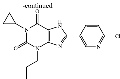
8-(6-Chloro-pyridin-3-yl)-1-cyclopropyl-3-propyl-3,7-dihydro-purine-2,6-dione
