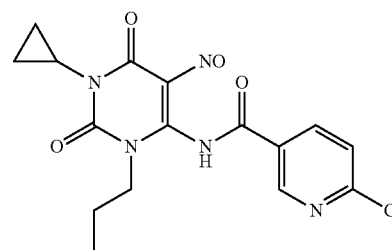
6-Chloro-N-(1-cyclopropyl-5-nitroso-2,6-dioxo-3-propyl-1,2,3,6-tetrahydro-pyrimidin-4-yl)-nicotinamide
