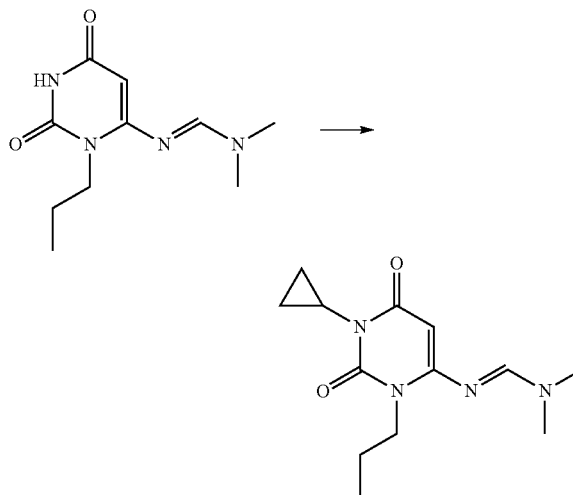
N-(1-Cyclopropyl-2,6-Dioxo-3-propyl-1,2,3,6-tetrahydro-pyrimidin-4-yl)-N,N-dimethyl-formamide
