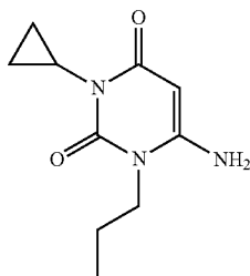
6-Amino-3-cyclopropyl-1-propyl-1H-pyrimidine-2,4-dione
