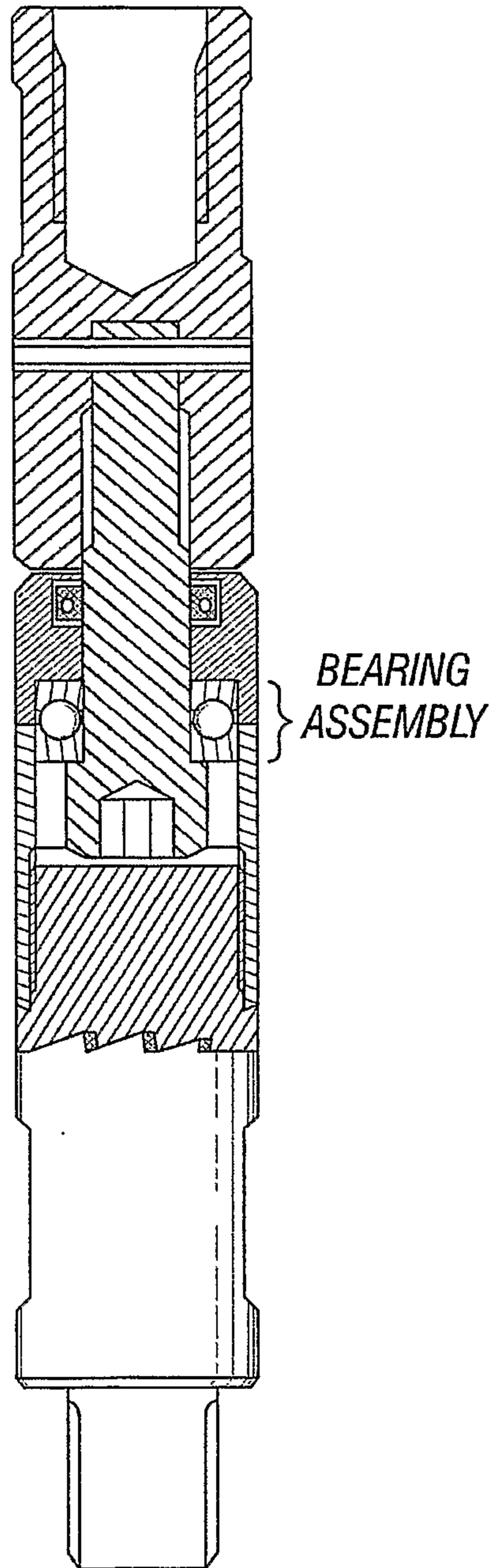
FIG. 3 (Prior Art)
