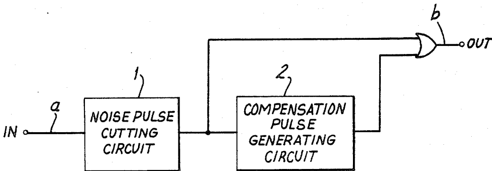
FIG. 3 PRIOR ART
