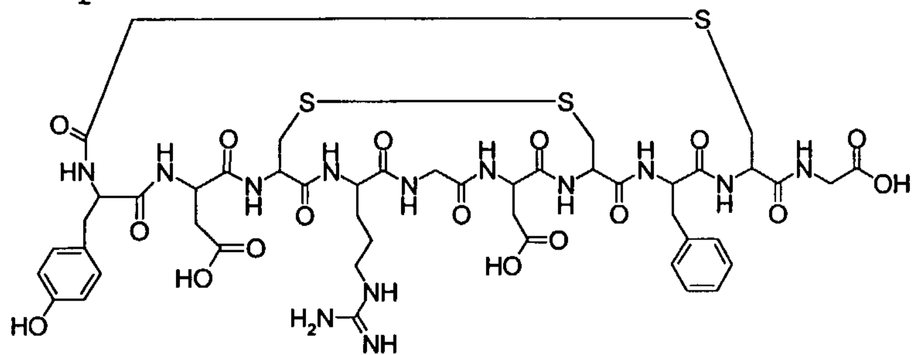
Compound III
