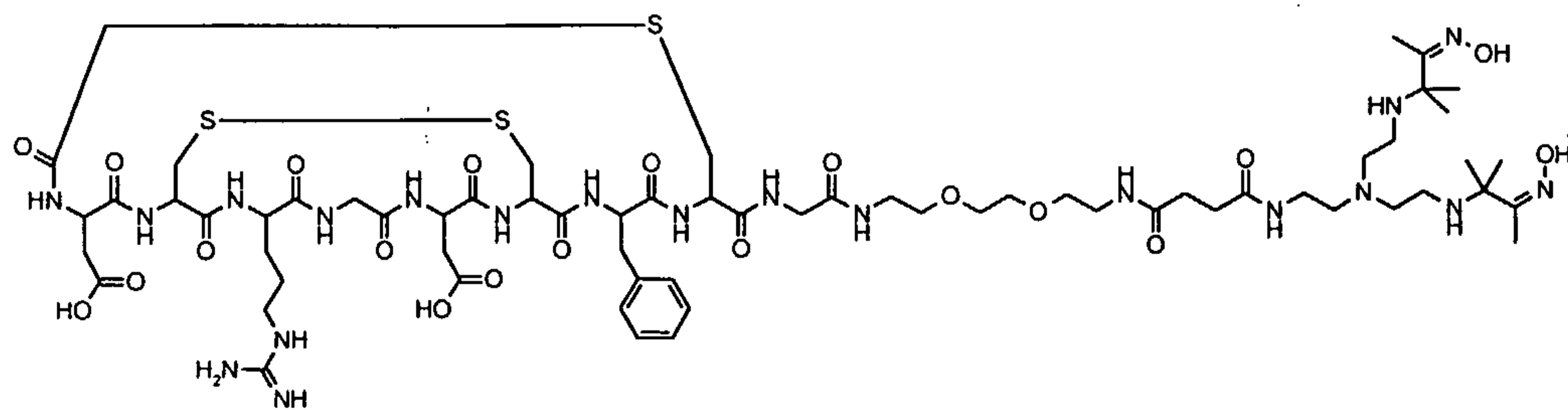
Compound V
