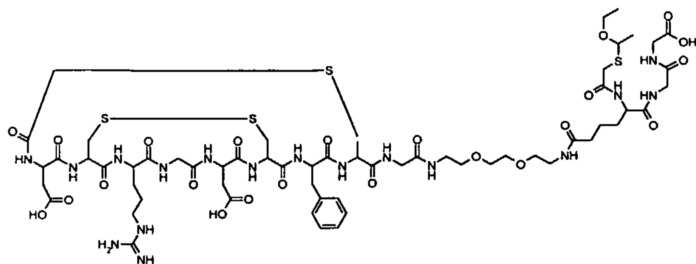
Compound VII
