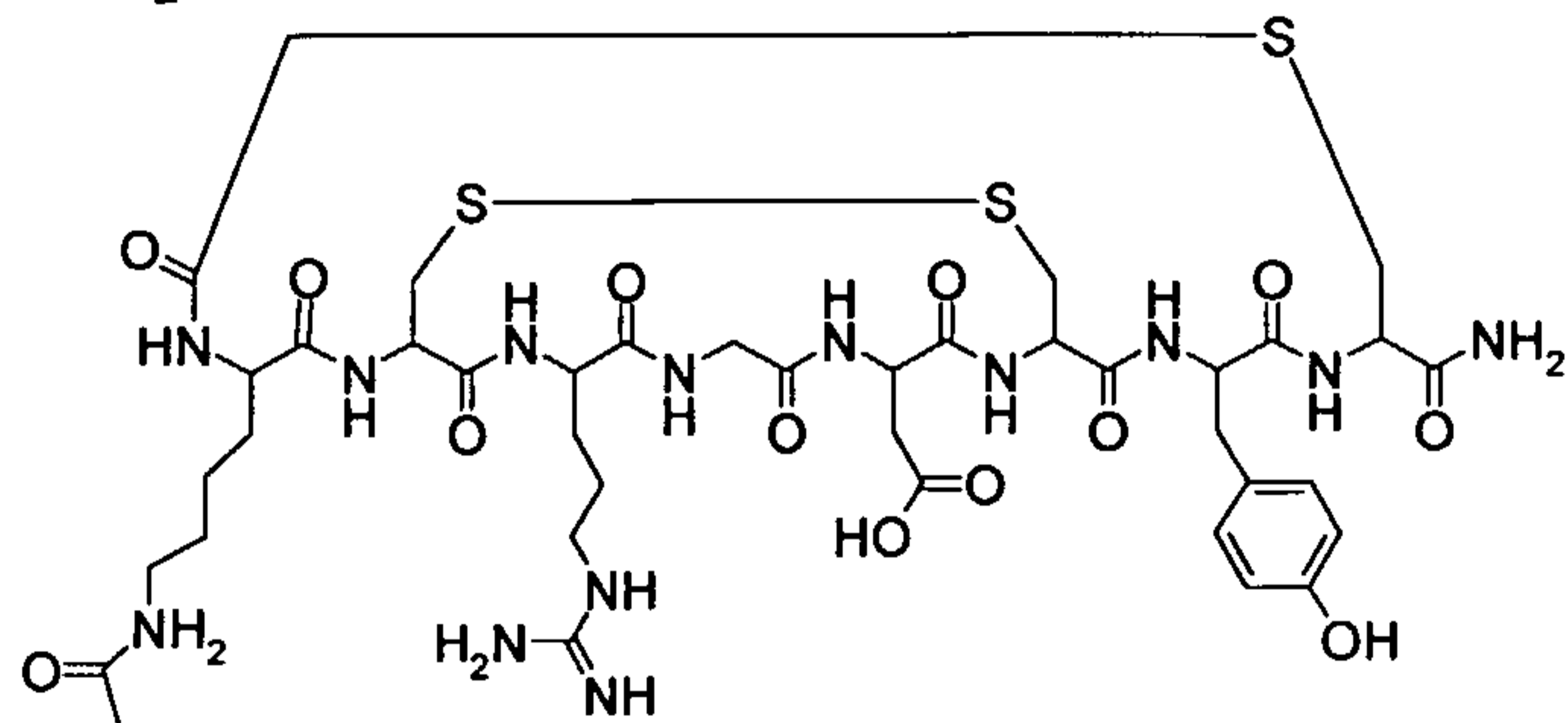
Compound IV
