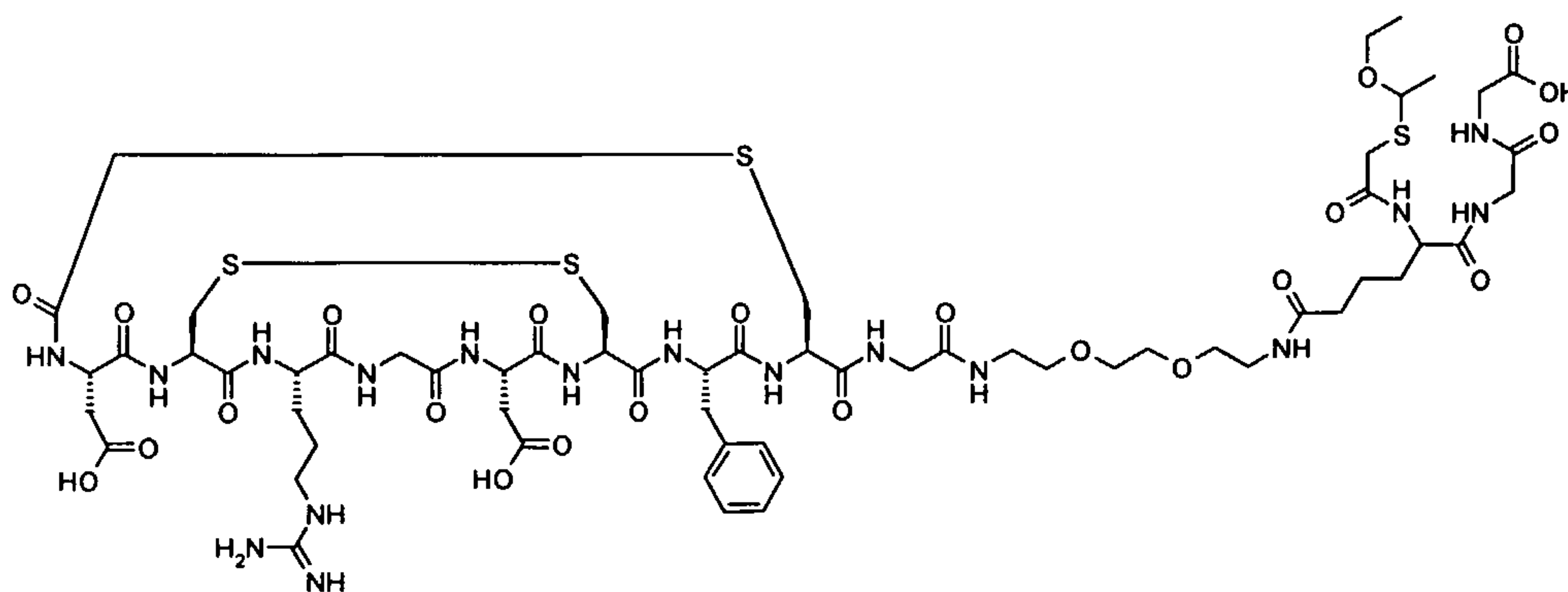
5 Compound VIa
