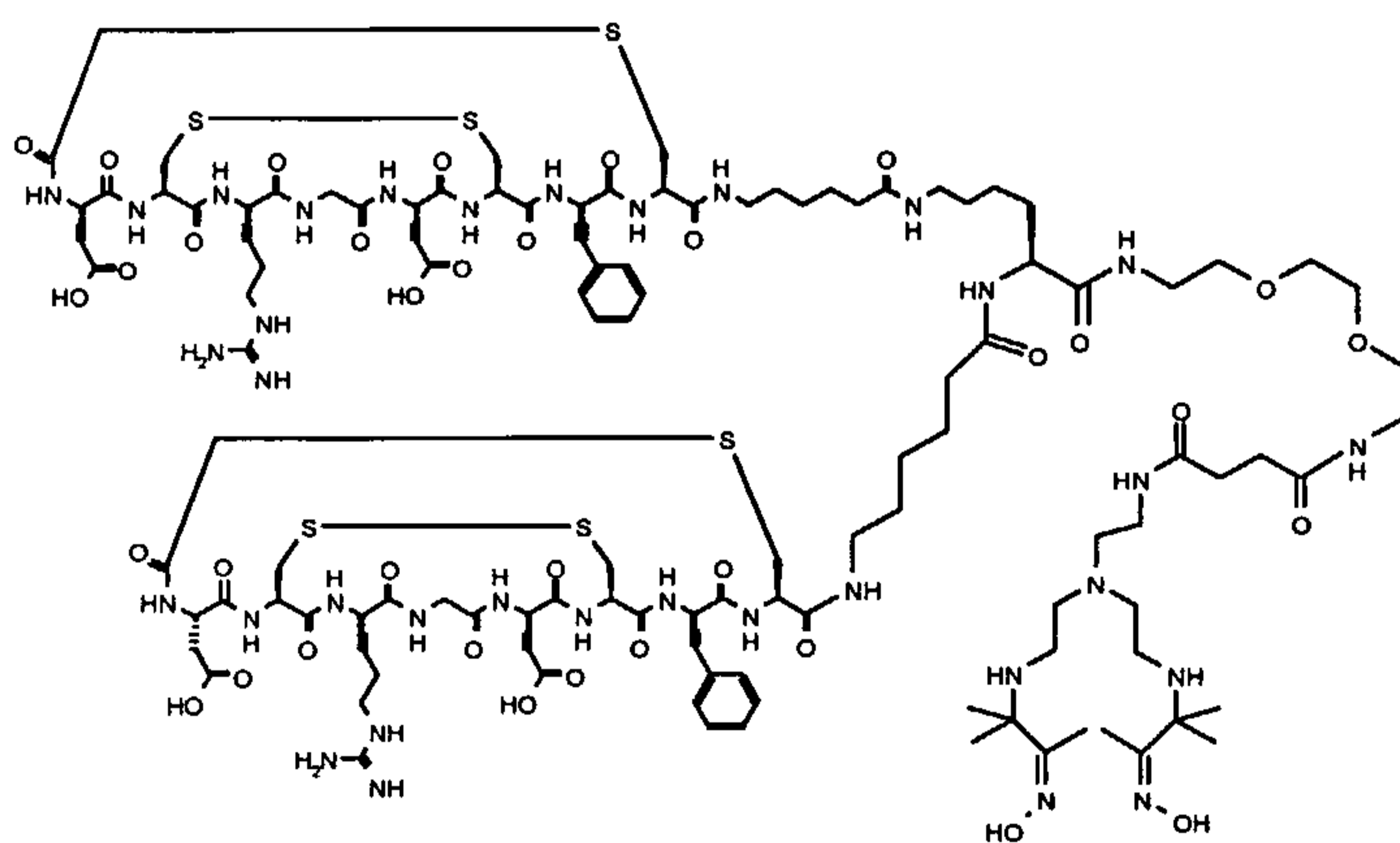
5 Compound VIII
