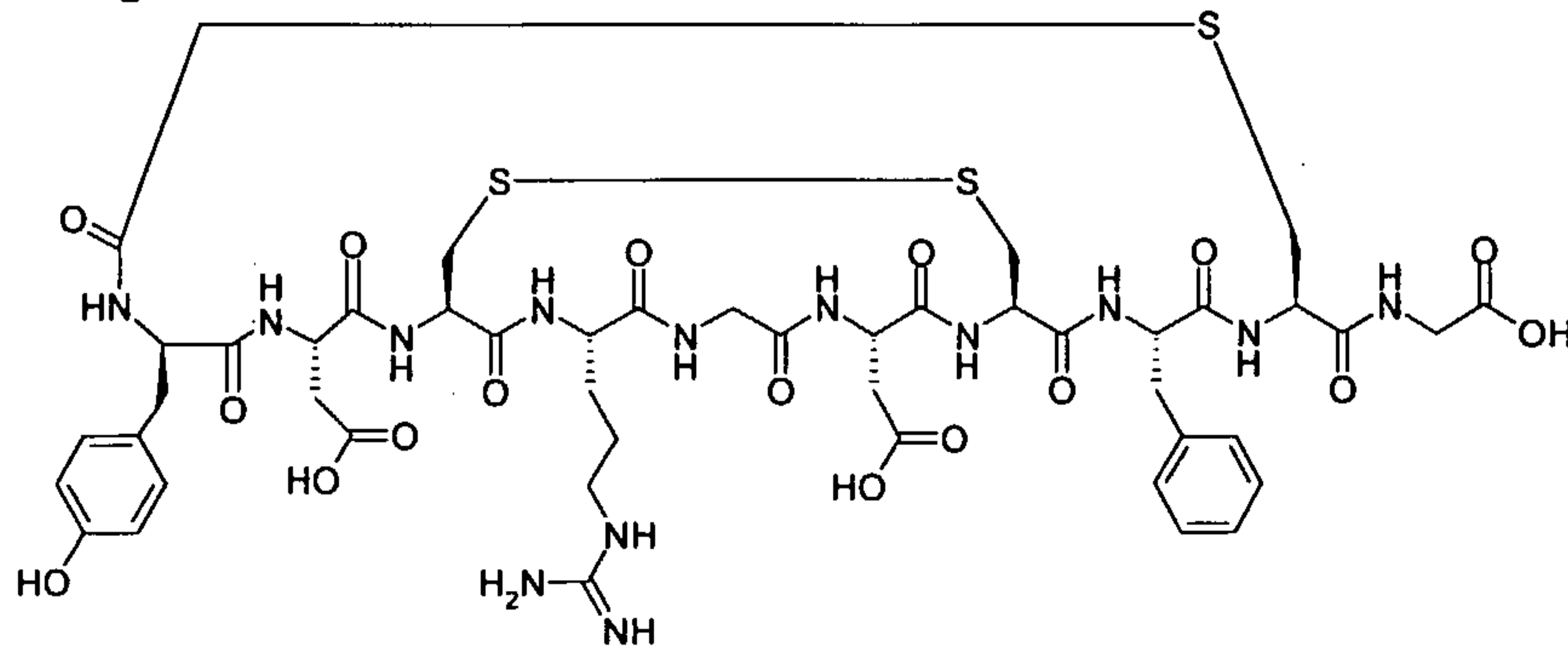
20 Compound IIIa
