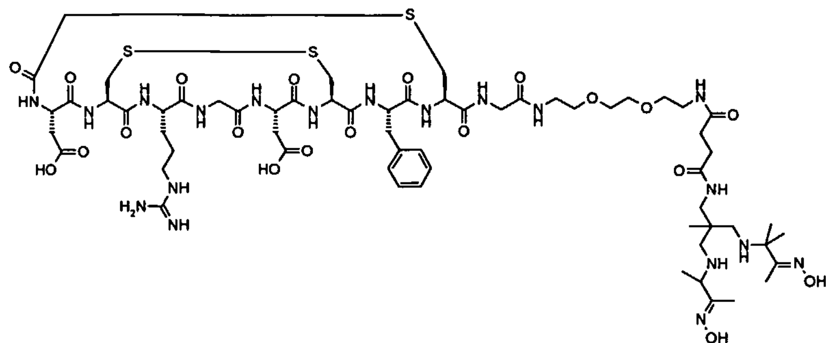
Compound IX
